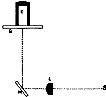
APPARATUS for measuring the duration of an electric spark.—S. Position of the spark. L. Achromatic lens. M. Revolving mirror. G. Glass plate for receiving the image of the spark. E. Telescope eye-piece.
